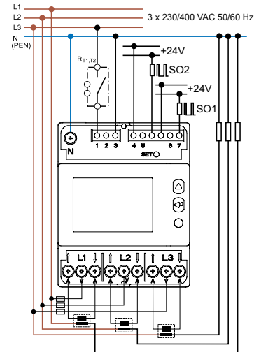
R_{T1,T2} = Tariff switching equipment
