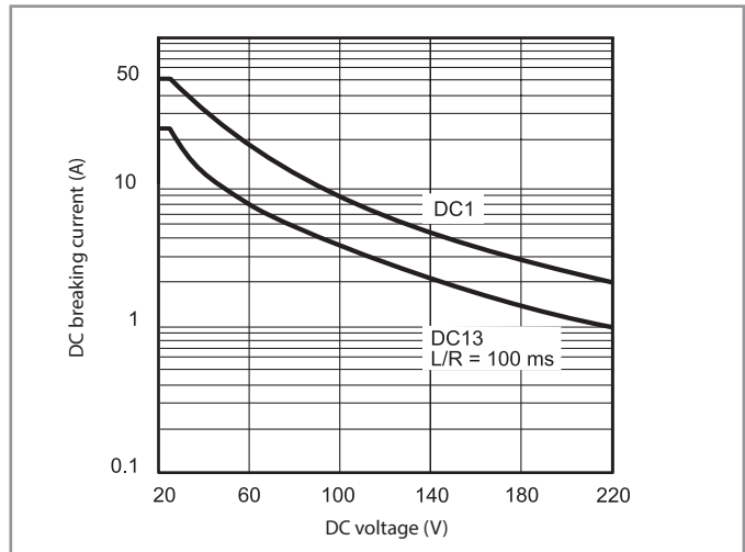
H 67-2 - Maximum DC breaking capacity (67.xx-x500)
