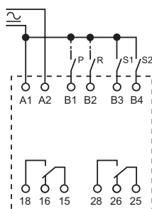
Wiring diagram
