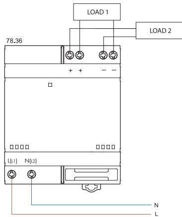
Basic connections
