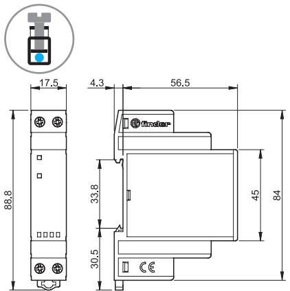
Type 77.01 DC Screw terminal
