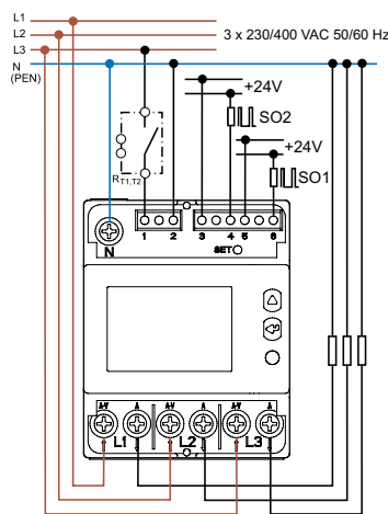
R_{T1,T2} = Tariff switching equipment
