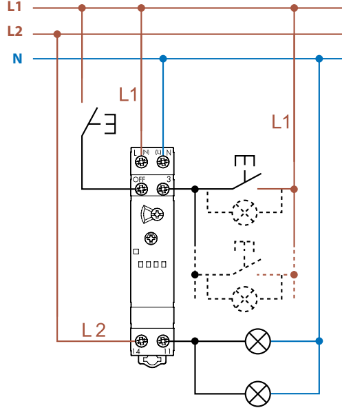
Type 14.11 Staircase light connection and load with different phases
